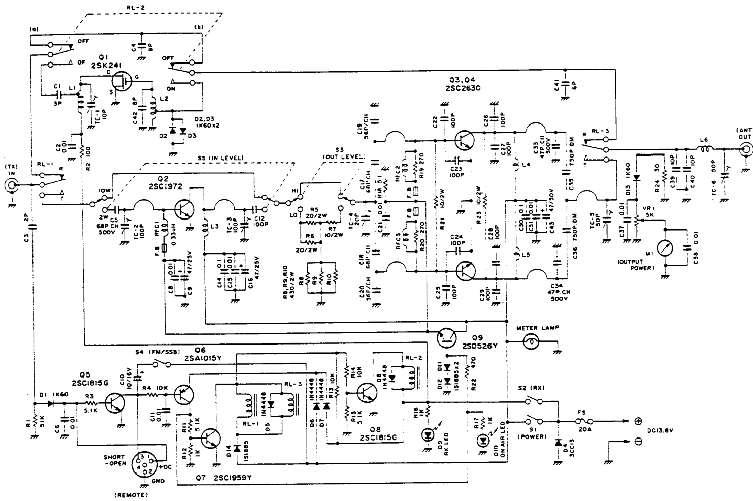
TOKYO HY-POWER HL-110V CIRCUIT DIAGRAM
